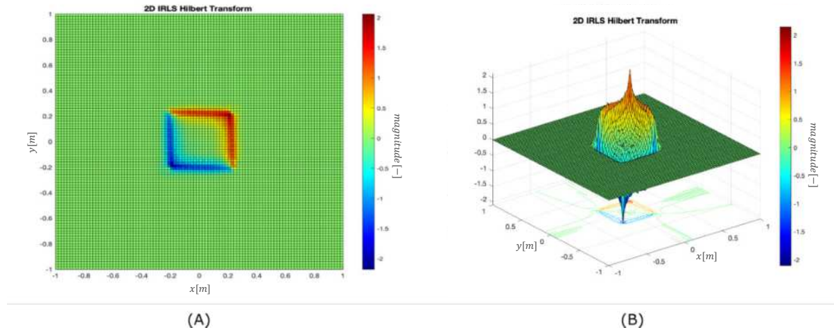
Figure 5-10: The 2D H-IRLS-HT of noisy dataset A) 2D view B) 3D view
