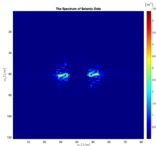
Figure 6-14: The spectrum of the noisy seismic data
